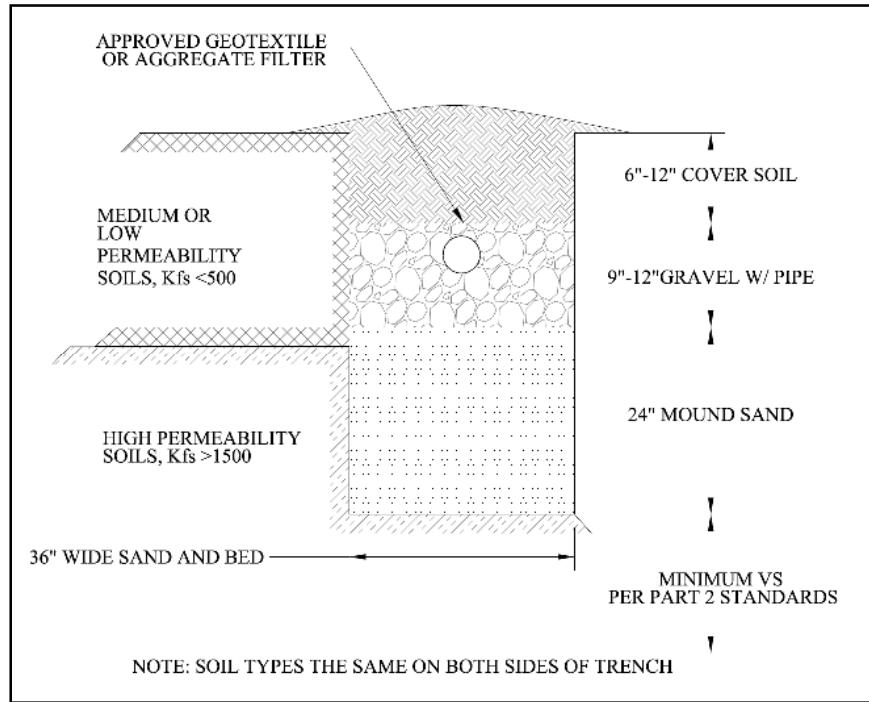
Figure 3-29 Sand-lined Trench
