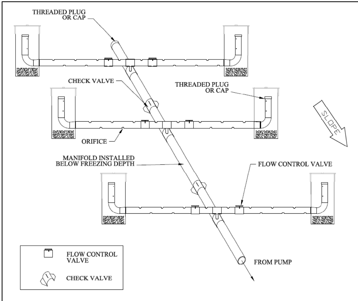
Figure 3-16 Tee to Tee Manifold, with Check Valves.
