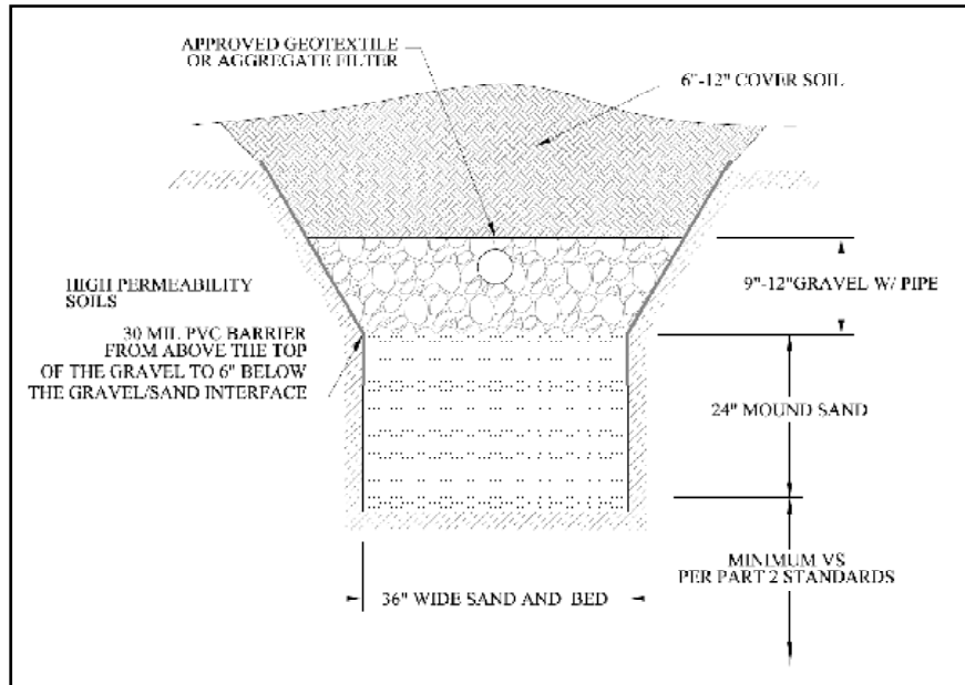
Figure 3-31 Sand-lined Trench with High Permeability Soils to Surface, Option 2
