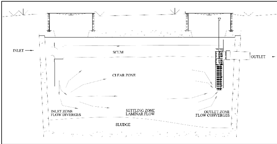
Figure 3-5 Flow in a Septic Tank.
