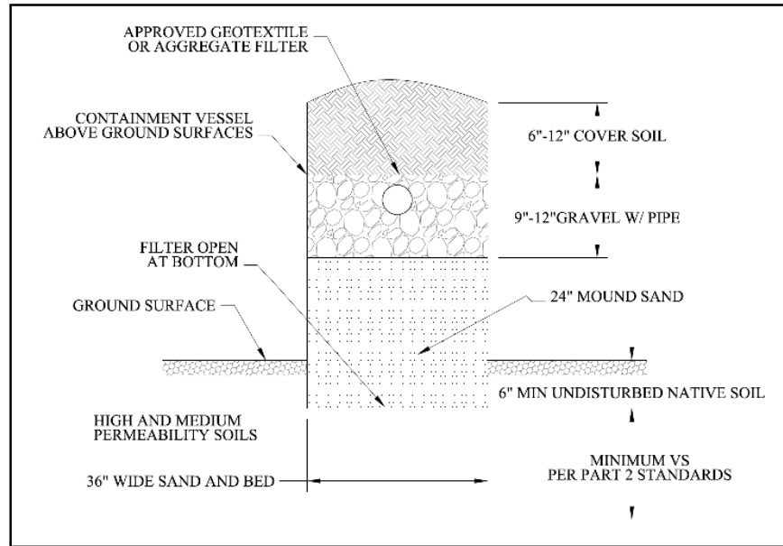
Figure 3-33 Above Ground Sand-lined Trench
