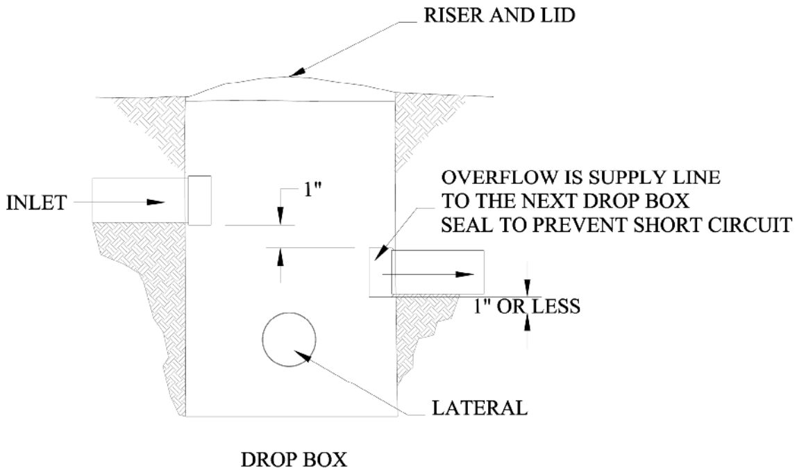
Figure 3-14 Sequential (Drop Box) System (Side View)
