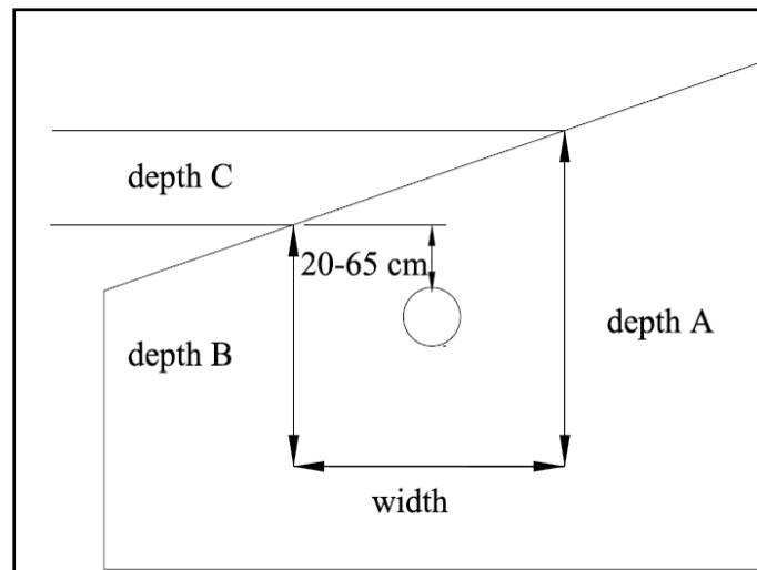
Figure 3-27 Trench Depth Variance on Sloped Site
