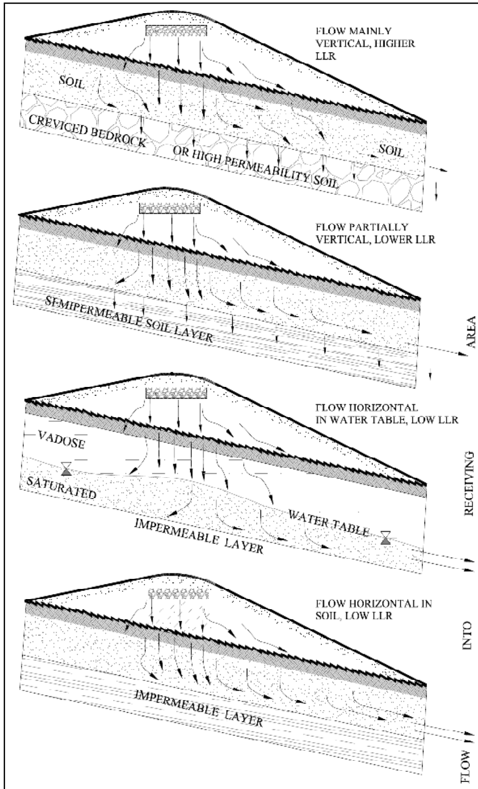
Figure 2-3 How Effluent Flows Away from a Discharge Area, and How this Affects LLR
