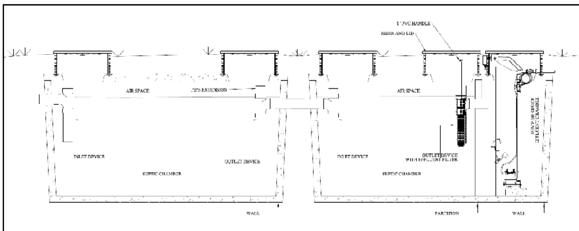
Figure 3-6 Septic Tank with Multiple Compartments Provided by Individual Tanks, and Pump Chamber in Third Compartment.
