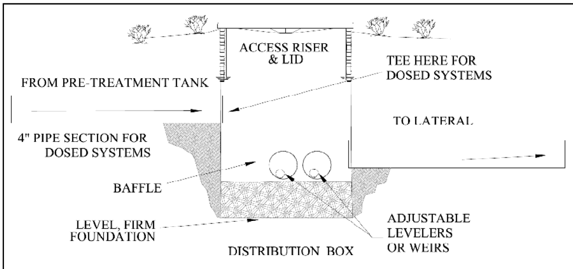
Figure 3-11 Distribution Box
