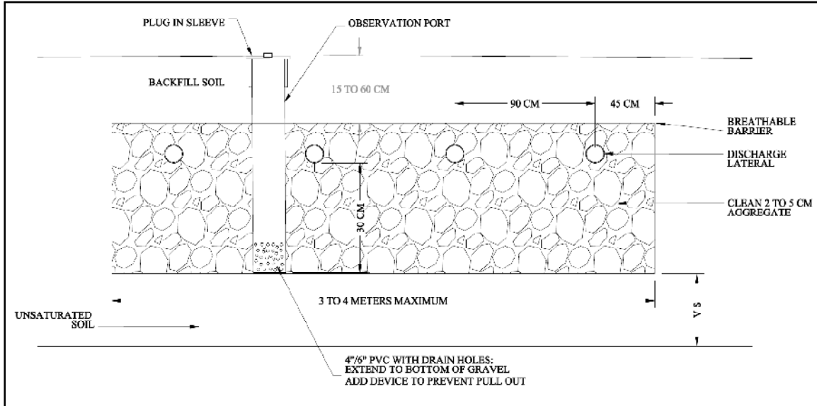
Figure 3-23 Seepage Bed Pressure Dispersal Typical Cross Section
