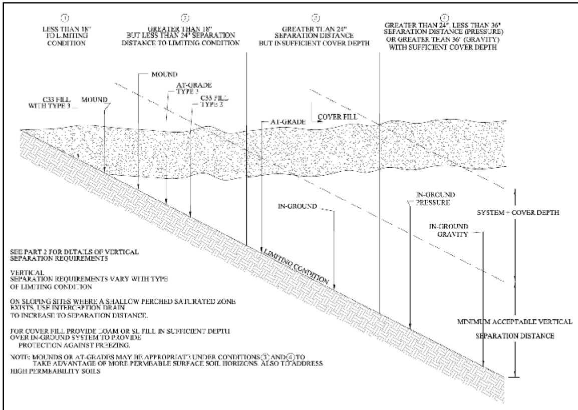
Figure 3-1 System Selection in Relation to Soil Depth
