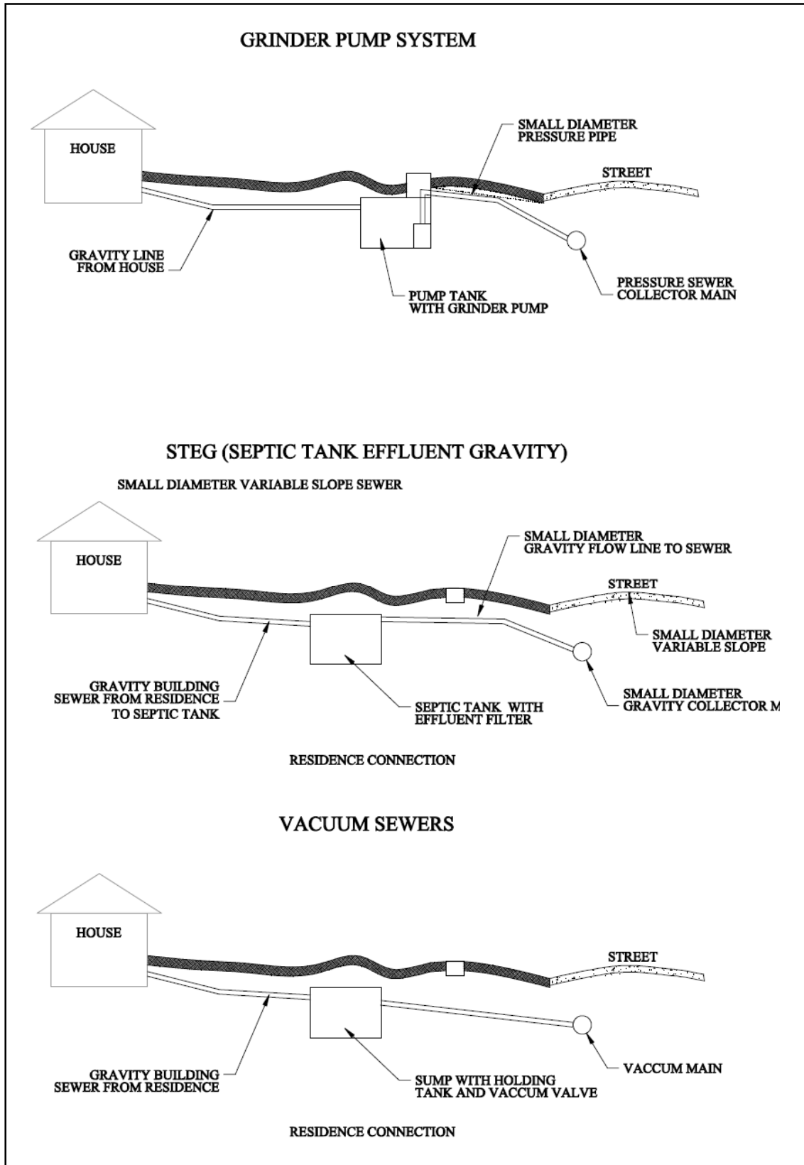
Figure 3-3 Diagram: Other Collector Systems, Showing Individual Connections
