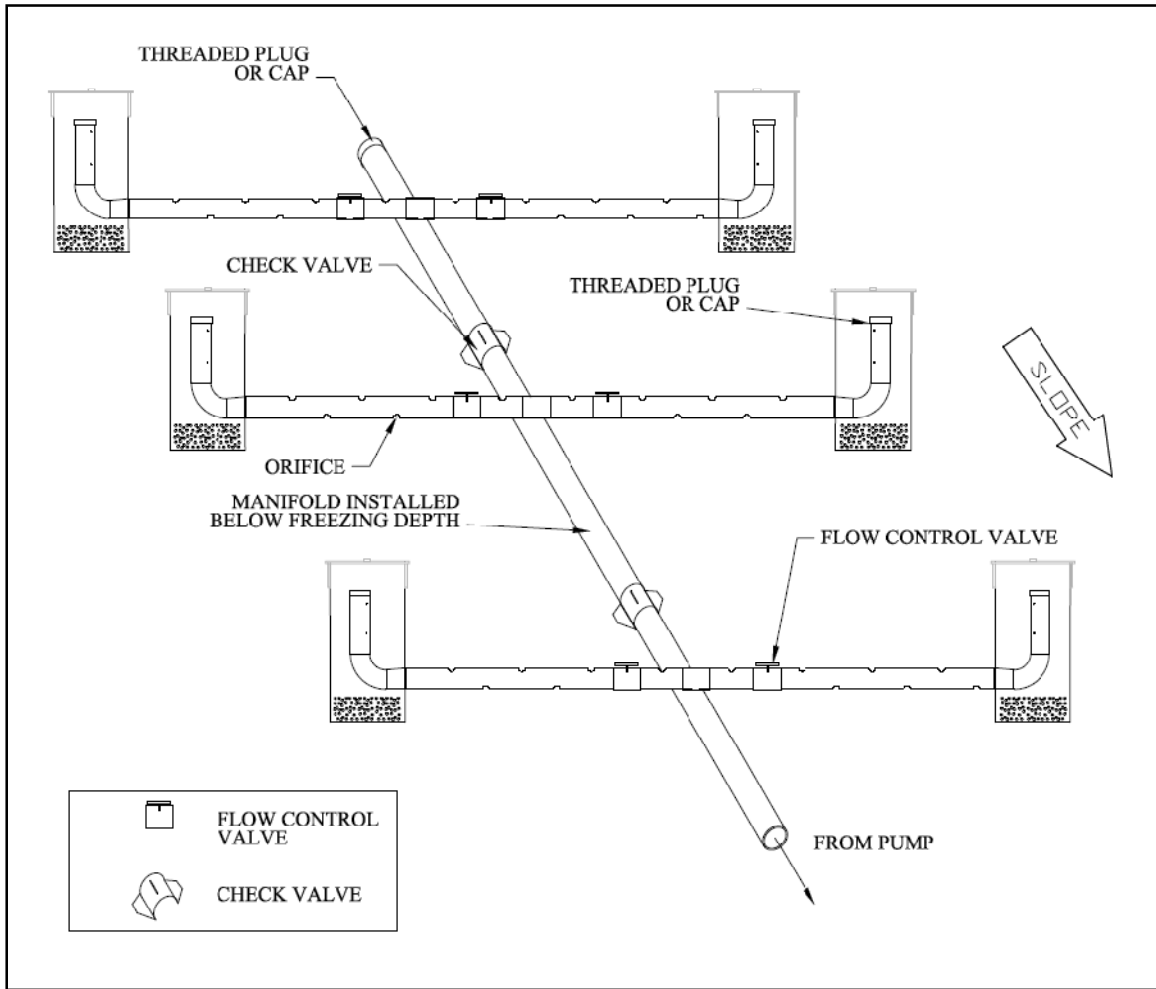
Figure 3-17 Cross Manifold, with Check Valves.
