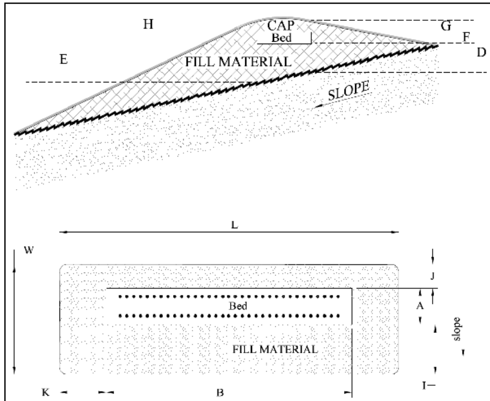
Figure 3-34 Mound Layout Schematic, Letter Dimensions Are as Used in the Worksheet.
