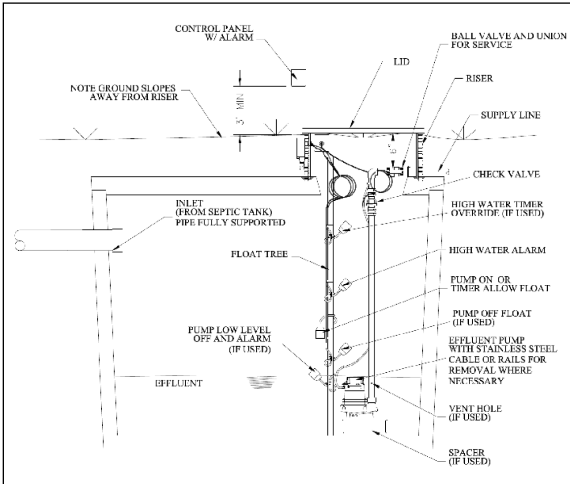
Figure 3-20 Pump Tank Nomenclature: Showing Piping Layout Suitable for Areas Where Heavy Frost Is Not Encountered.
