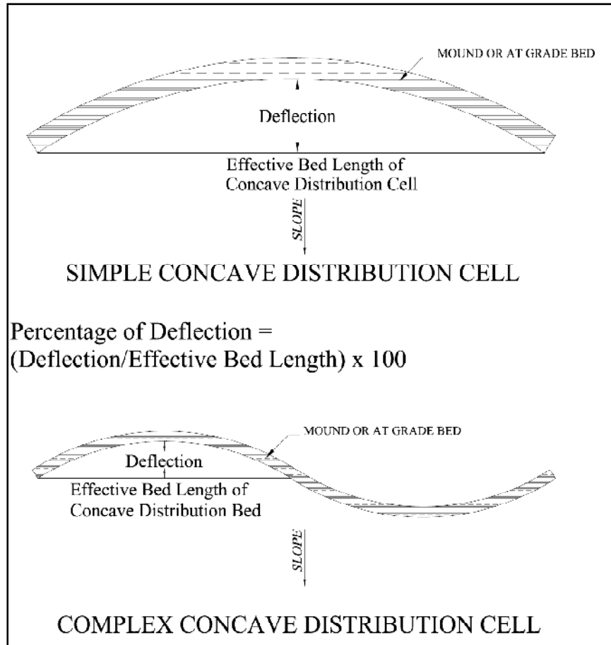
Figure 3-36 Calculation of Effective Bed Length on Site with Concave Contour
