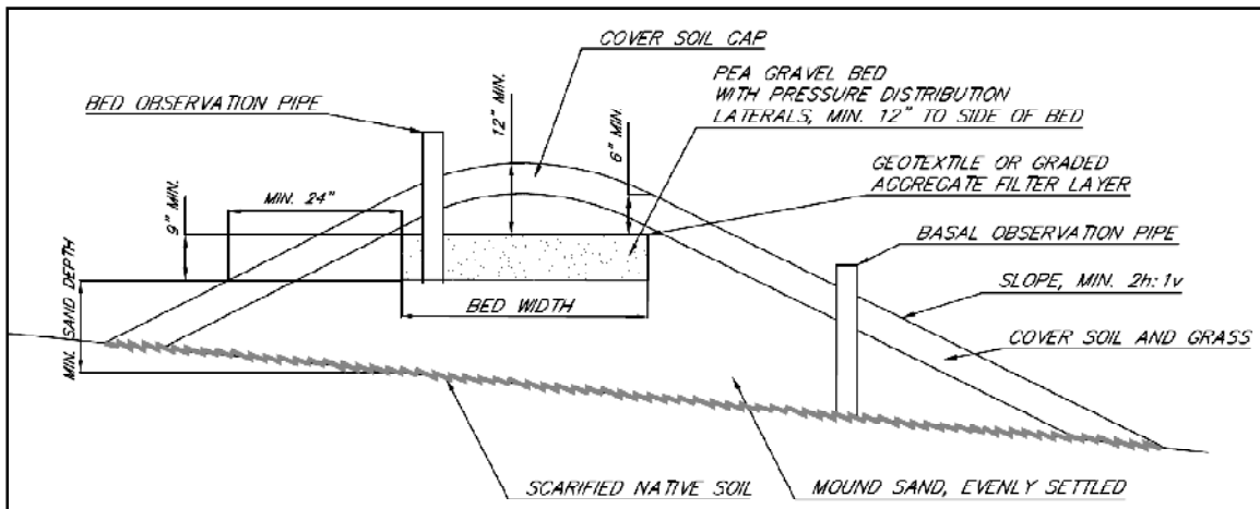
Figure 3-28 Example of a Mound Cross Section Showing Nomenclature
