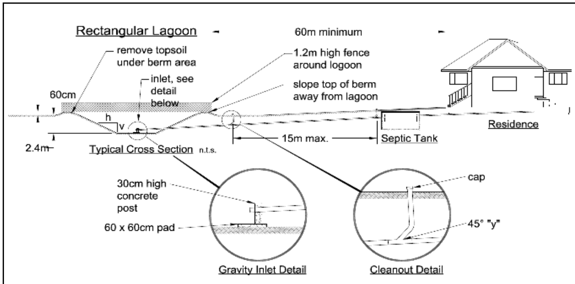
Figure 3-37 Rectangular Lagoon
