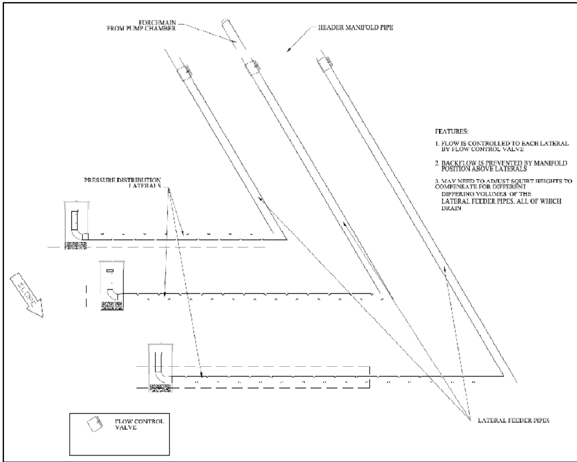
Figure 3-18 Short Upslope Header Manifold, with Feeder Pipes to Laterals.
