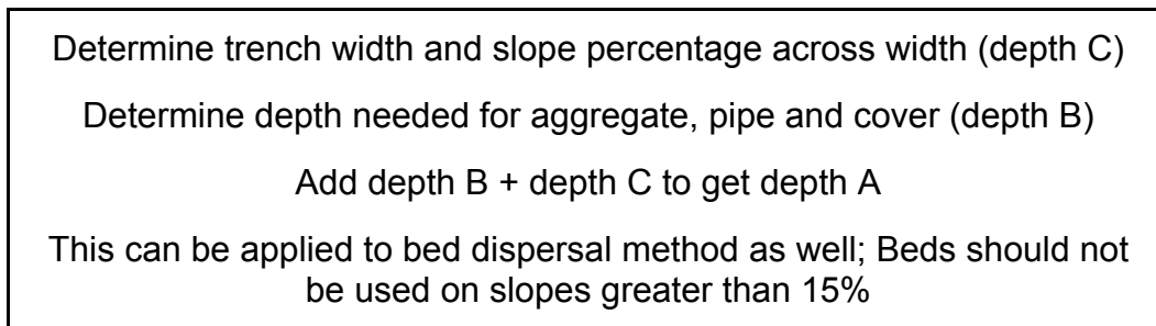
Figure 3-27 Trench Depth Variance on Sloped Site
