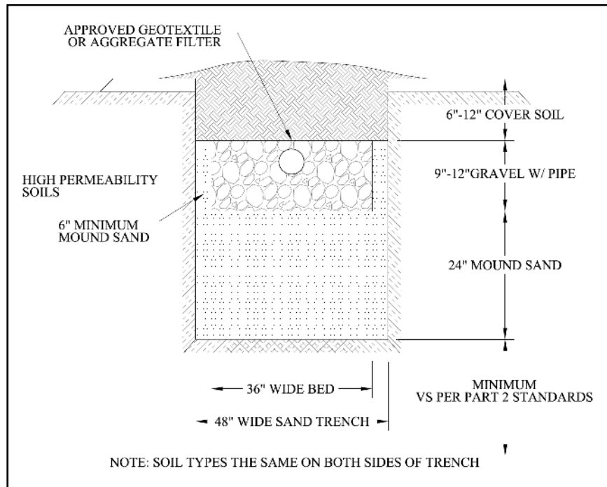
Figure 3-30 Sand-lined Trench with High Permeability Soils to Surface, Option 1
