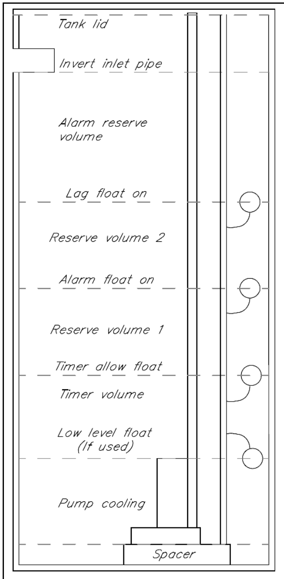
Figure 3-22 Schematic of Timed Dosing Terms: Showing Example of Tank with Lag Float
