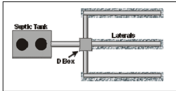
Figure 3-10 Gravity Trench Distribution
