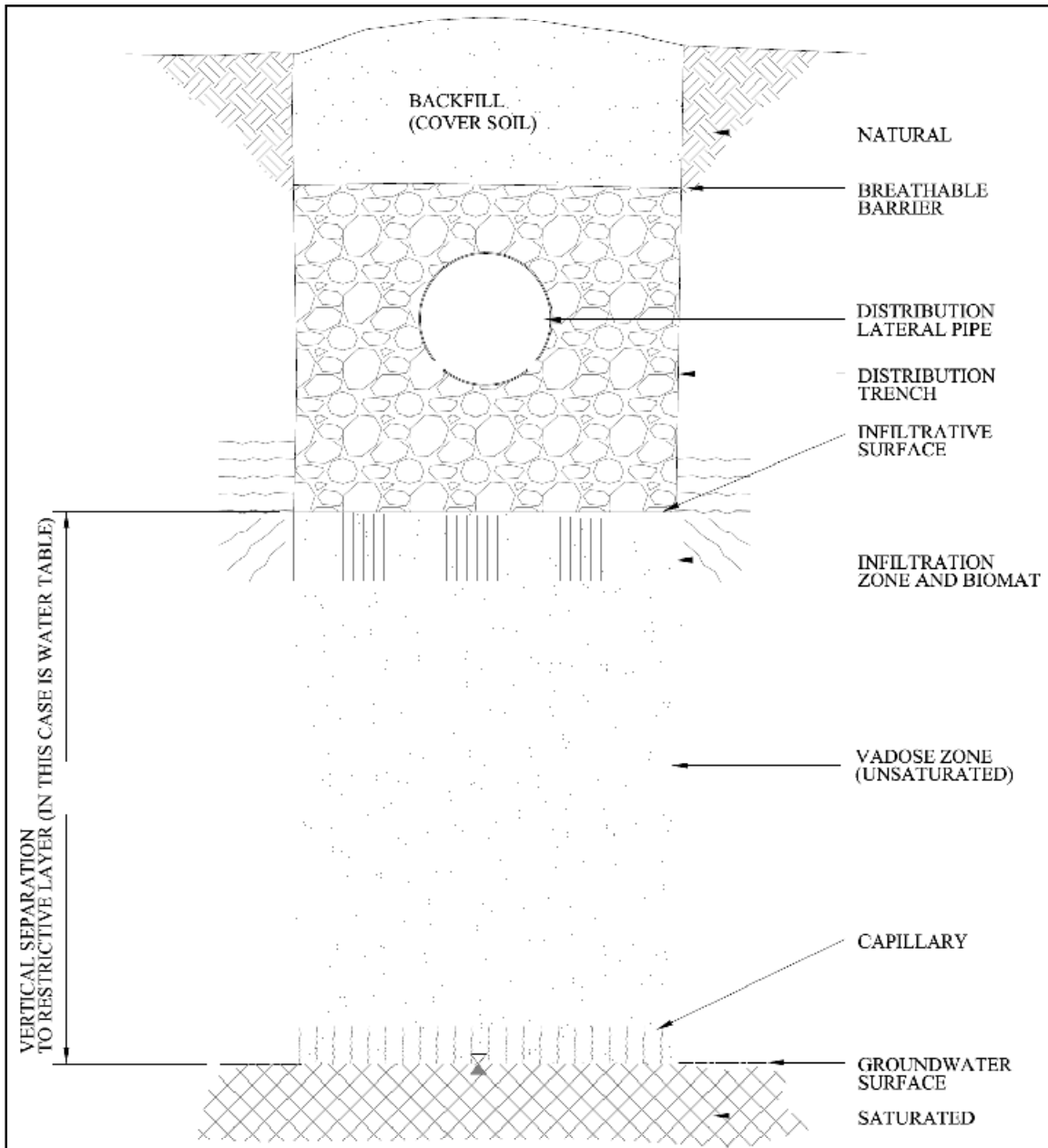
Figure 2-1 Vertical Separation between the Infiltrative Surface and the Restrictive Layer.
