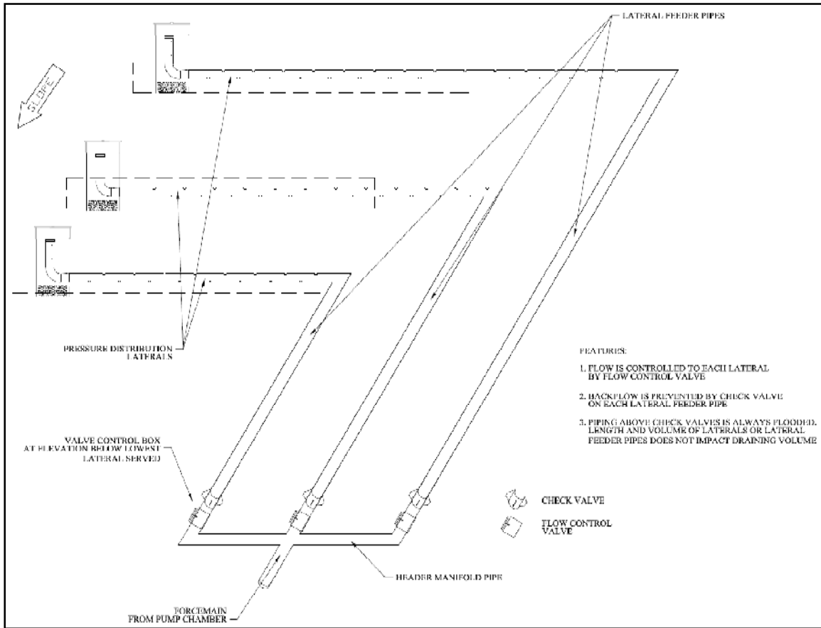
Figure 3-19 Short Downslope Header Manifold, with Check Valves.
