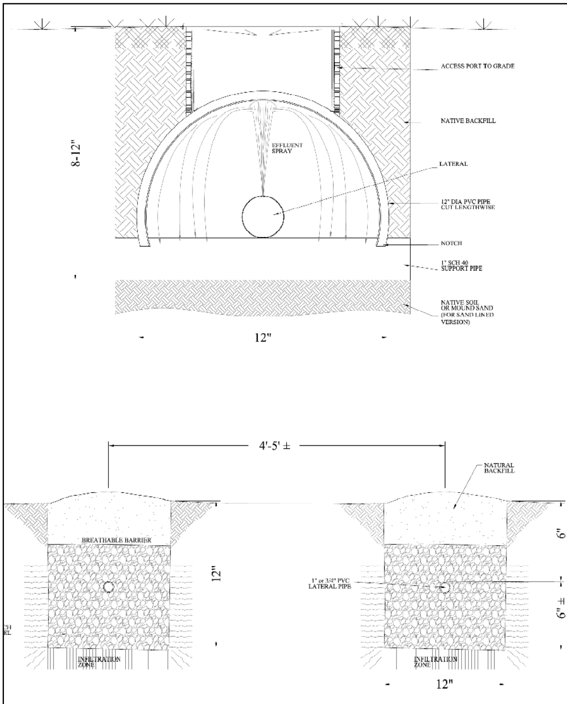
Figure 3-25 Shallow Narrow Drainfield Cross Sections
