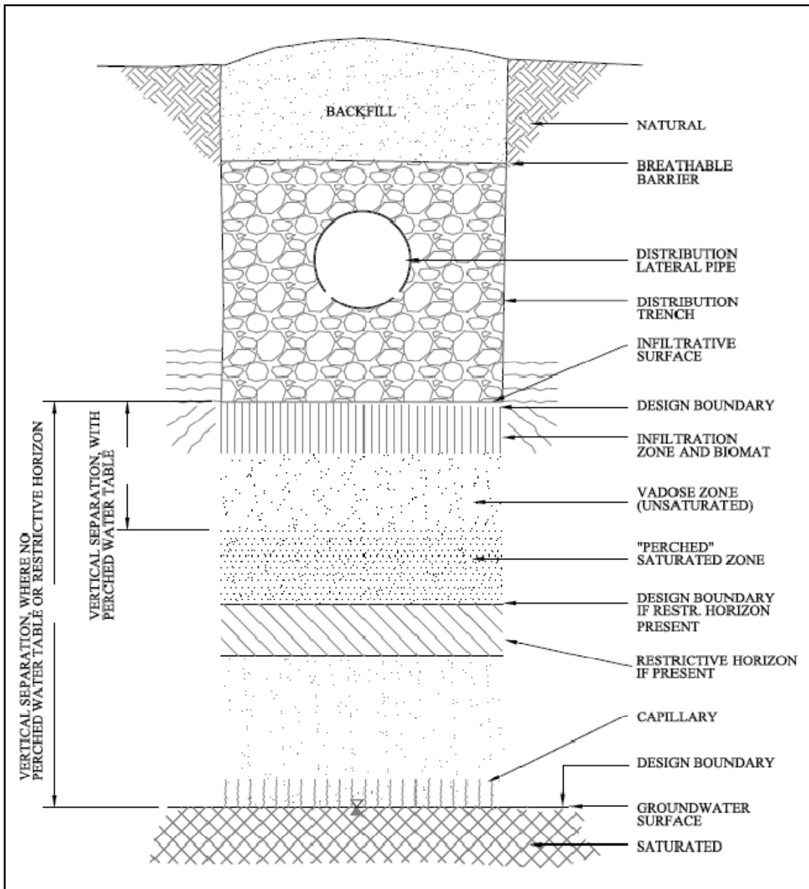
Figure 3-7 A SWIS Trench System, Showing Terminology
