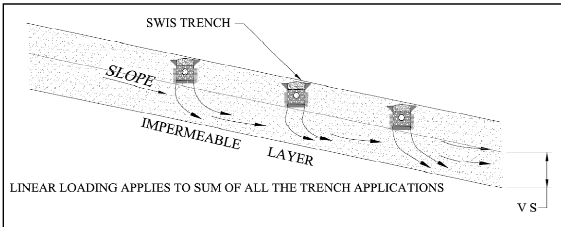
Figure 2-2 Linear Loading Rate on a Slope, Showing Trench Cross Sections
