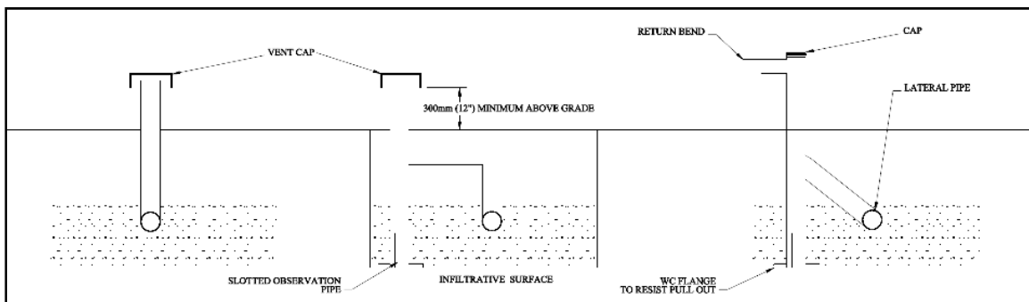
Figure 3-9 Vent and Combination Vent and Observation Port Examples
