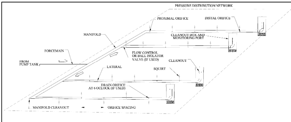
Figure 3-15 Pressure Distribution System
