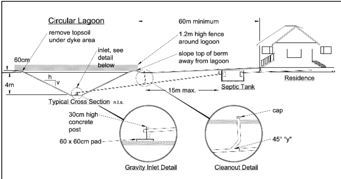
Figure 3-39 Circular Lagoon
