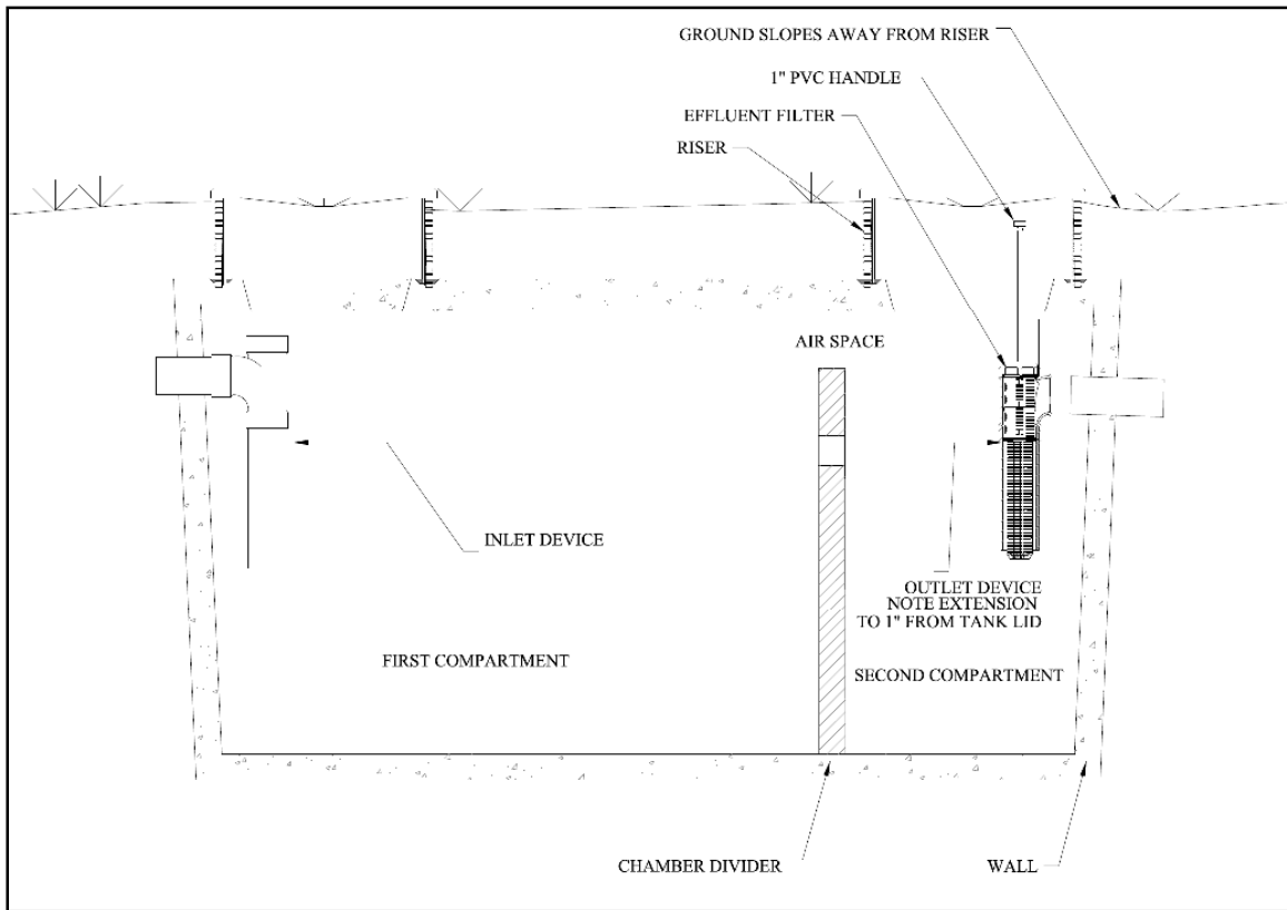
Figure 3-4 Compartmentalized Septic Tank.
