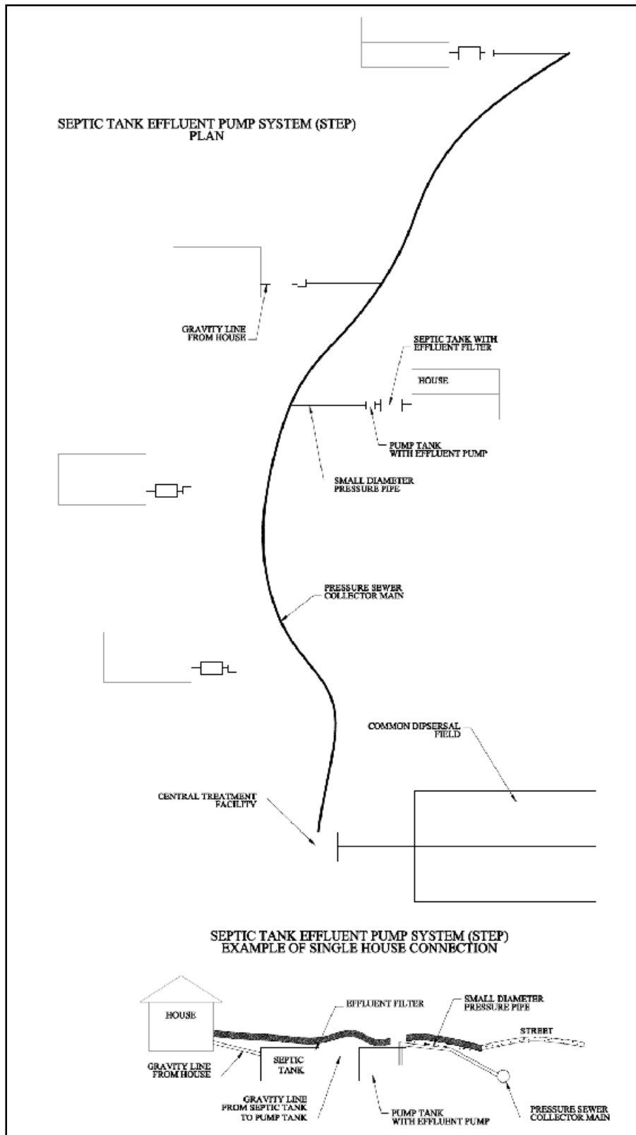
Figure 3-2 Diagram: STEP System Schematic Plan and Individual Connection
