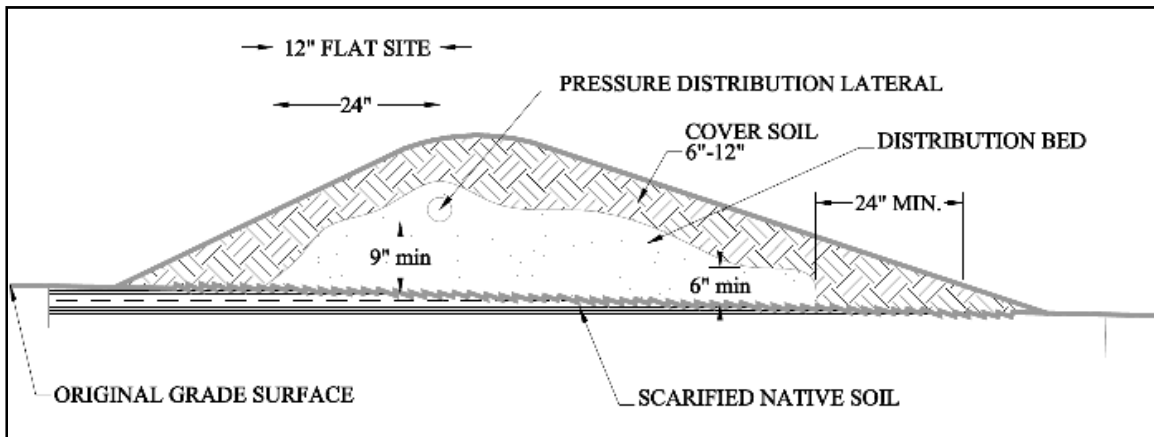
Figure 3-24 At Grade Bed Typical Cross Section
