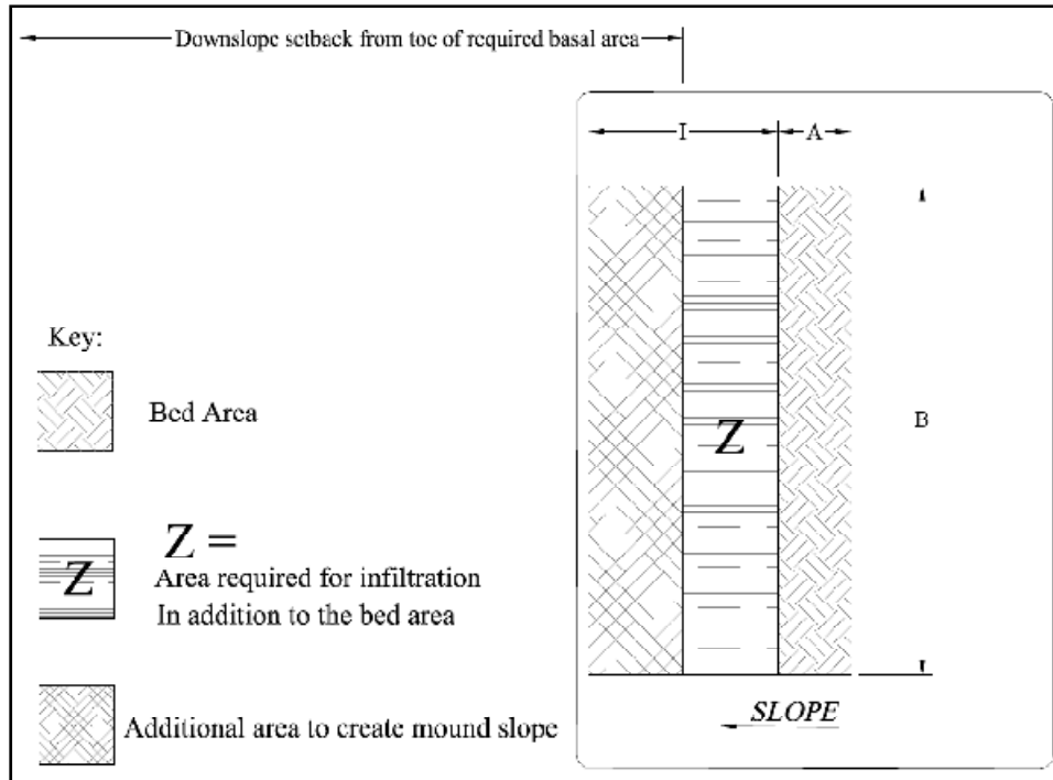
Figure 3-35 Horizontal Setbacks are Measured from the Edge of the Minimum Basal Area of the Mound
