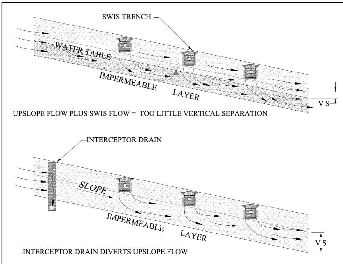
Figure 3-26 Use of an Interception Drain
