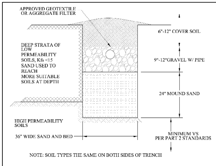
Figure 3-32 Sand-lined Trench to Reach Suitable Soil at Depth
