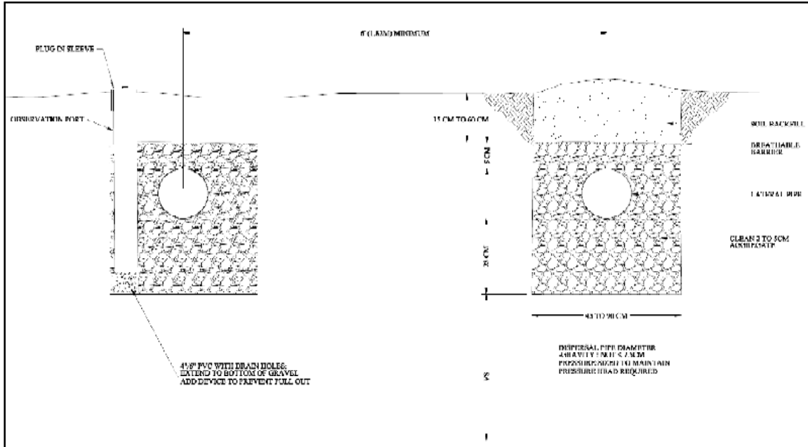
Figure 3-8 Trench Dispersal Layout
