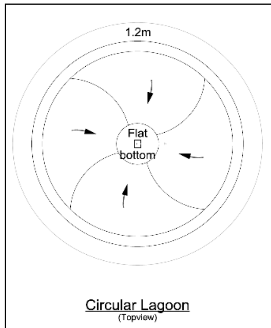
Figure 3-40 Circular Lagoon (Top View)
