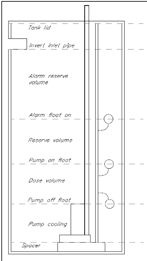
Figure 3-21 Schematic of Demand Dosing Terms
